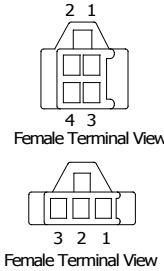
Female Terminal View
